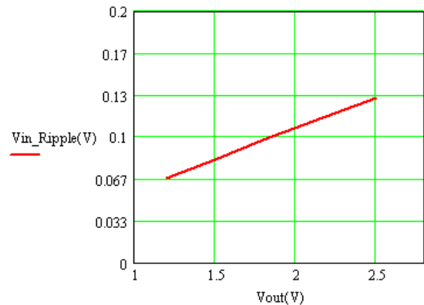
Figure 26: Input ripple voltage for various output models, I_o = 3A ( C_{in} = 2 \times 100\mu F electrolytic capacitors, 1 \times 3.3\mu F ceramic capacitors at the input)
