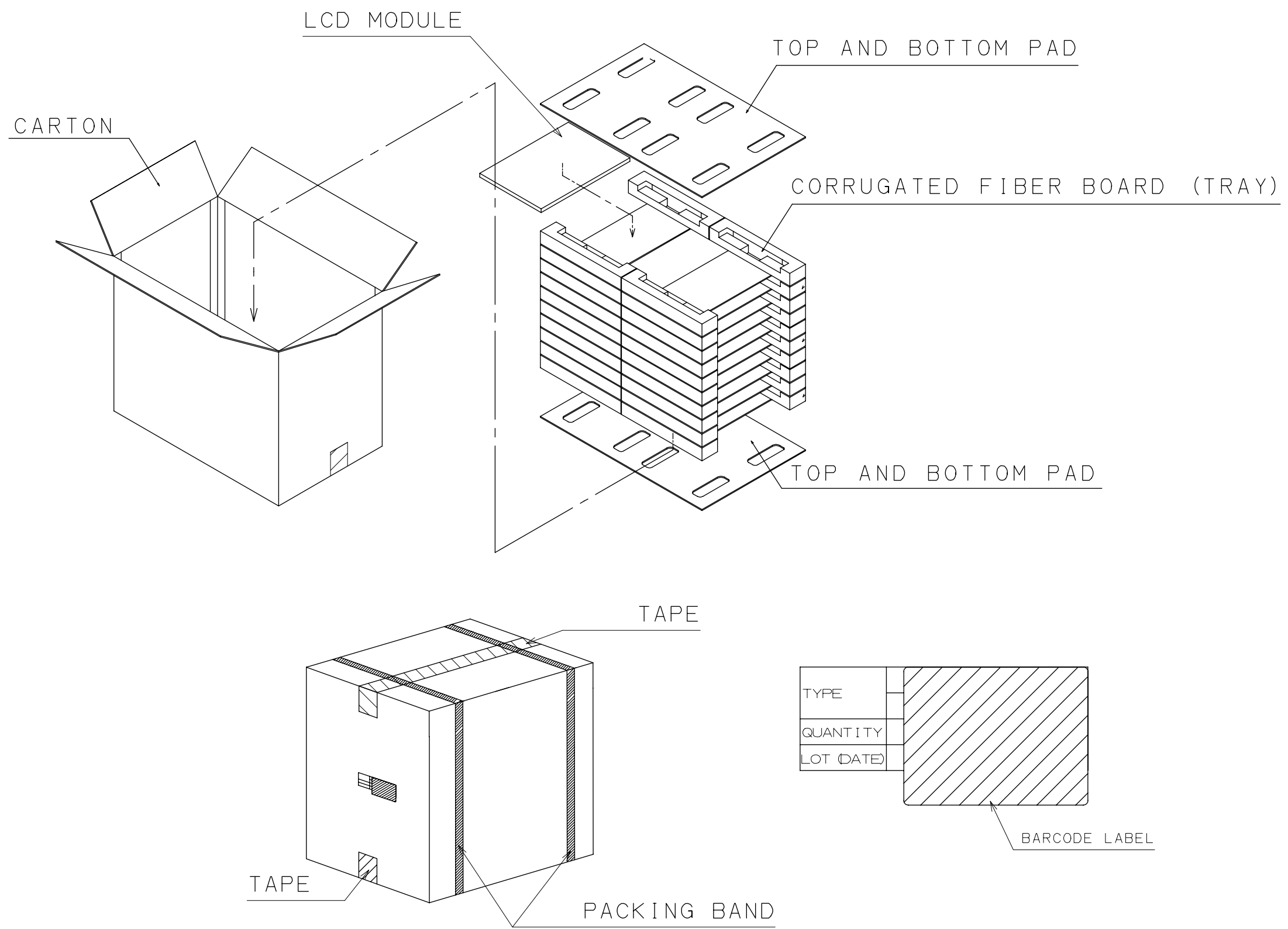
FIG. 3:PACKING FORM
