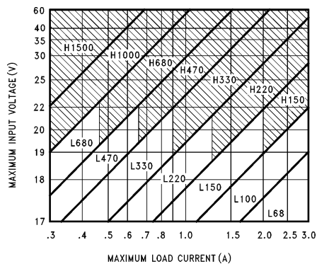
FIGURE 6. LM2576(HV)-15
