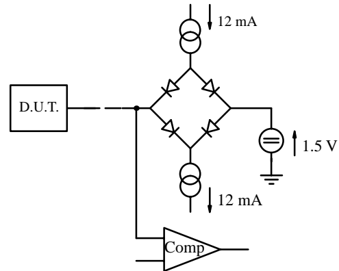
Figure 5. Typical ULC Test Conditions
