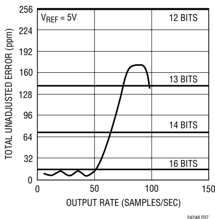
Figure 7. Total Error vs Output Rate ( V_{\text{REF}} = 5\text{V} )
