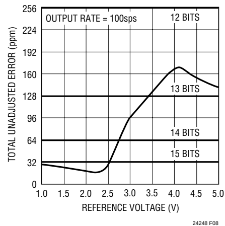
Figure 8. Total Error vs V_{\text{REF}} (Output Rate = 100sps)
