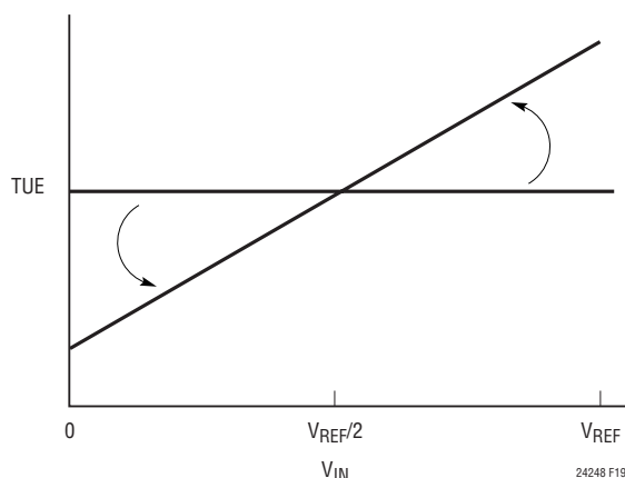
Figure 19. Offset/Full-Scale Shift
