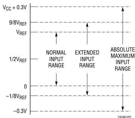
Figure 2. LTC2424/LTC2428 Input Range
