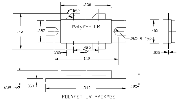
PACKAGE DIMENSIONS IN INCHES
