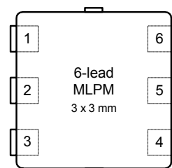
Figure 2. Package Type
