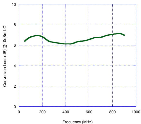
Figure 10. Conversion Loss vs. Frequency
