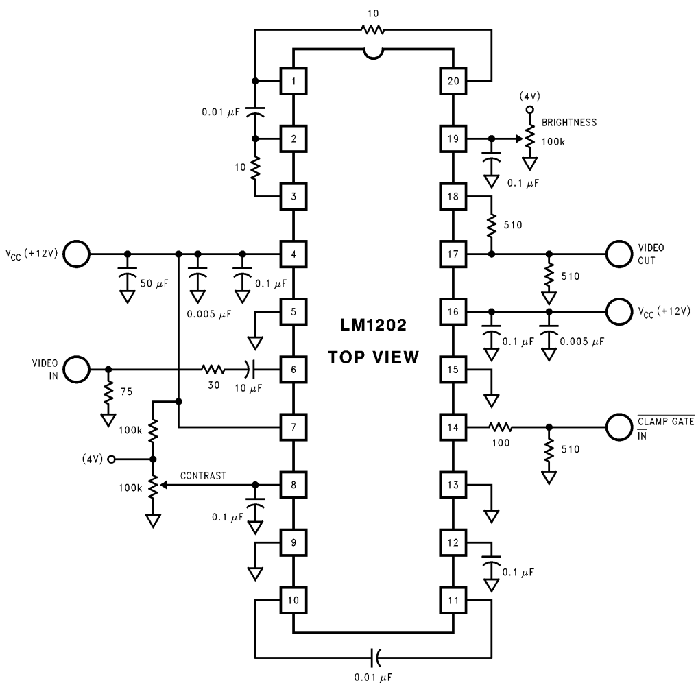
FIGURE 9. Typical LM1202 Application (Single Video Channel)
