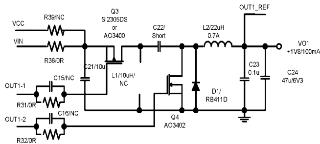
POWER CH2(SEPIC)
