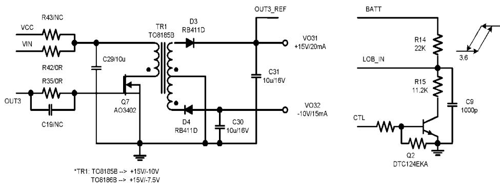
POWER CH3 (FLYBACK)
