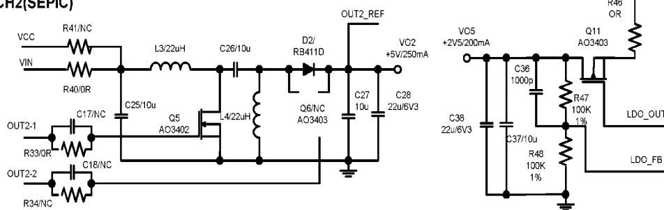
POWER CH2(SEPIC)
