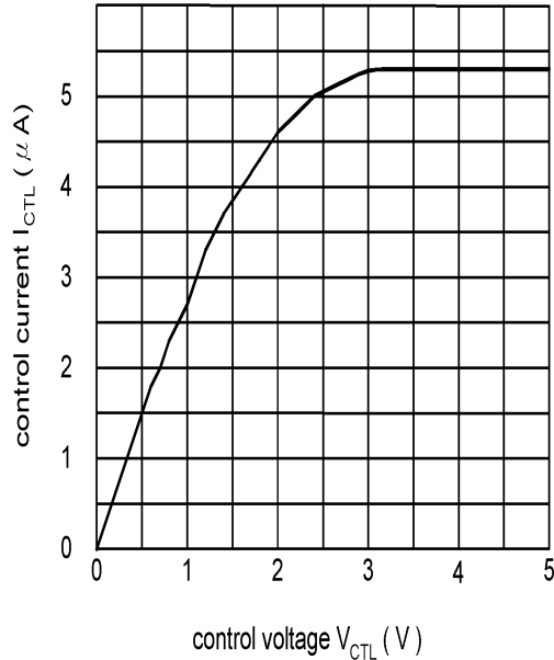
control voltage vs. control current (CTL)
