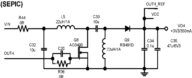
POWER CH1(STEP-DOWN)
