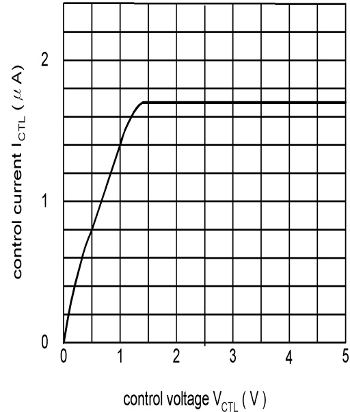
control voltage vs. control current (CTL1-CTL4)
