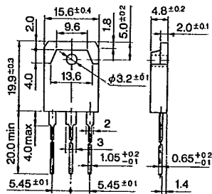
Outline Drawing ⑨
