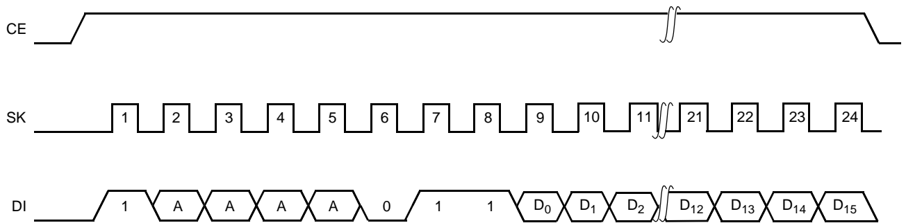
Figure 2. RAM Write
