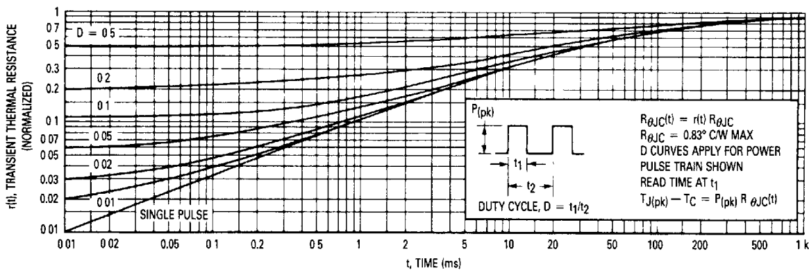
Figure 10. Thermal Response
