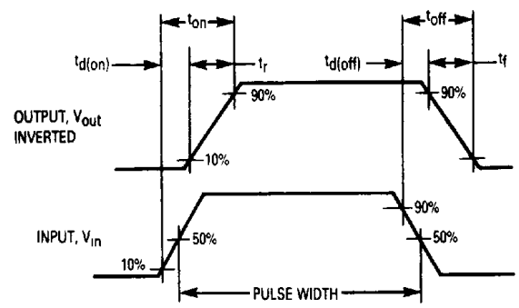
Figure 14. Switching Waveforms
