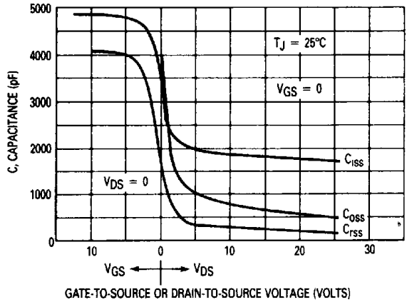
Figure 11. Capacitance Variation
