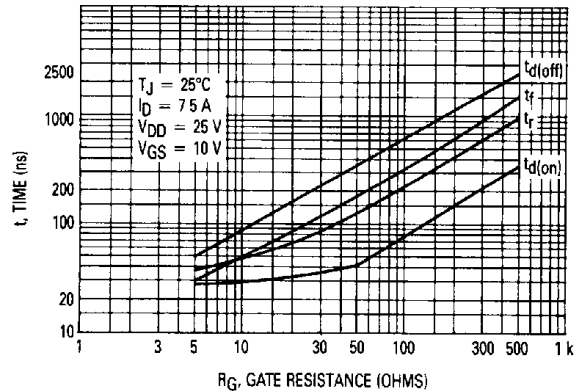
Figure 9. Resistive Switching Time Variation With Gate Resistance
