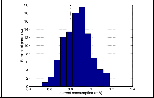
Figure 19. Current consumption at 3.3V
