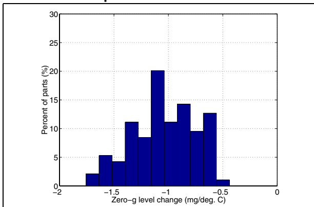
Figure 13. z-axis Zero-g level change Vs temperature
