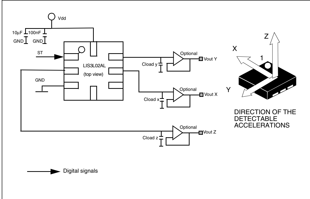
Figure 3. LIS3L02AL Electrical Connection
