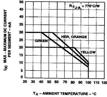
Figure 10. Maximum Allowable DC Current vs. Ambient Temperature.
