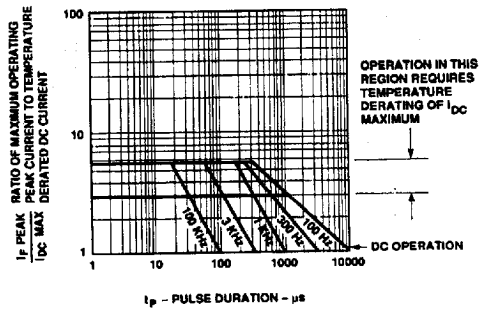
Figure 8. Maximum Tolerable Peak Current vs. Pulse Duration - Yellow.
