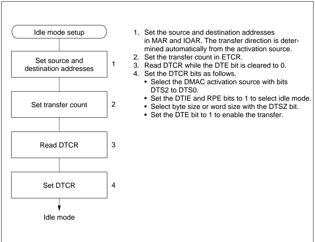
Figure 8-5 Idle Mode Setup Procedure (Example)
