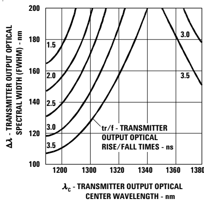
HFBR-5803 FDDI TRANSMITTER TEST RESULTS OF \lambda_c , \Delta\lambda AND t_r/f ARE CORRELATED AND COMPLY WITH THE ALLOWED SPECTRAL WIDTH AS A FUNCTION OF CENTER WAVELENGTH FOR VARIOUS RISE AND FALL TIMES.
