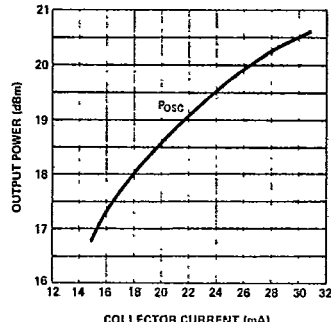
Figure 12. Typical Oscillator Power vs. Collector Current for V_{CE} = 15 V at 4.3 GHz, for the HXTR-4101.
