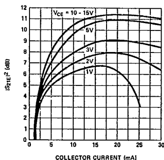
Figure 8. Typical |S_{21}|^2 vs. Collector Current at 2 GHz, for the HXTR-6106.
