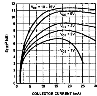
Figure 6. Typical |S_{21}|^2 vs. Collector Current at 2 GHz, for the HXTR-2102.
