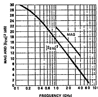
Figure 3. Typical MAG, and |S_{21}|^2 vs. Frequency ( V_{CE} = 15\text{ V} , I_C = 25\text{ mA} ), for the HXTR-2102.
