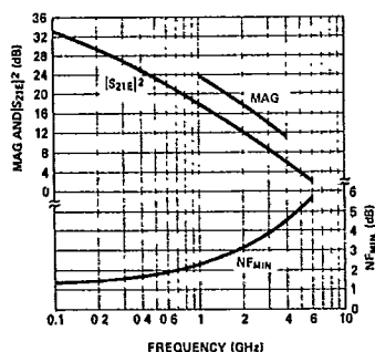
Figure 1. Typical MAG, |S_{21}|^2 , and Noise Figure ( NF_{MIN} ) vs. Frequency ( V_{CE} = 15\text{ V} , I_C = 25\text{ mA} ), for the HXTR-2001.
