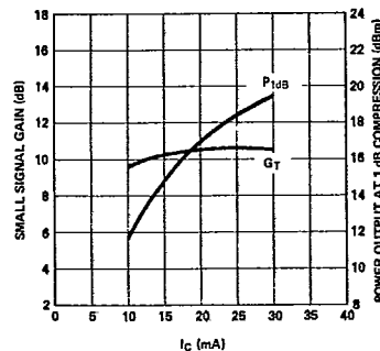
Figure 5. Typical |S_{21}|^2 vs. Collector Current at 4 GHz, for the HXTR-2101.
