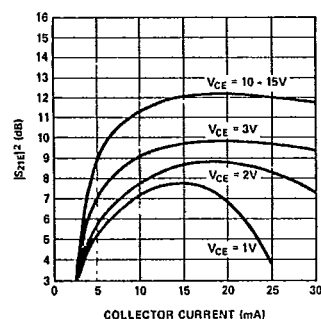
Figure 4. Typical |S_{21}|^2 vs. Current at 2 GHz, for the HXTR-2001.
