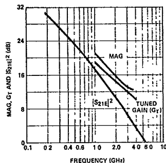
Figure 2. Typical MAG, |S_{21}|^2 , and Tuned Gain vs. Frequency ( V_{CE} = 15\text{ V} , I_C = 25\text{ mA} ), for the HXTR-2101.
