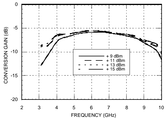
Unconverter Performance Conversion Gain vs. LO Drive
