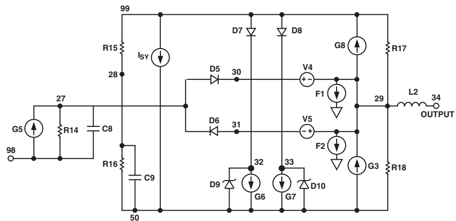
Figure 19c. Spice Diagram
