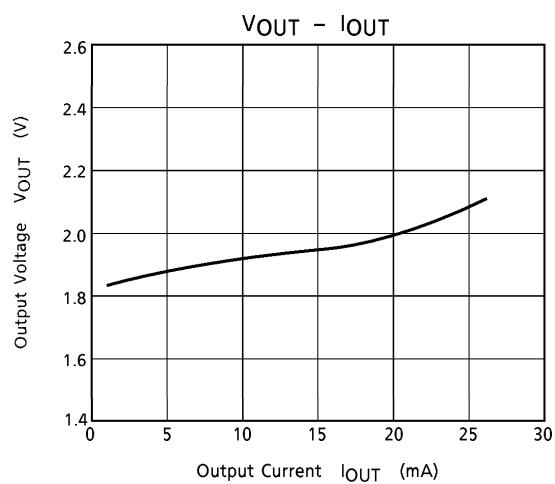
(2) Output Voltage Characteristic ( V_{OUT} )
