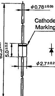
Outline Drawing ④
