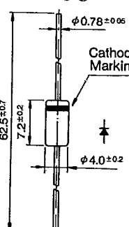
Outline Drawing ⑤
