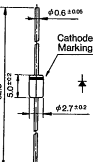
Outline Drawing ③
