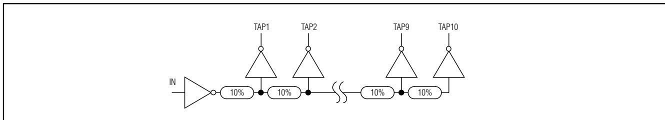
Figure 1. Logic Diagram
