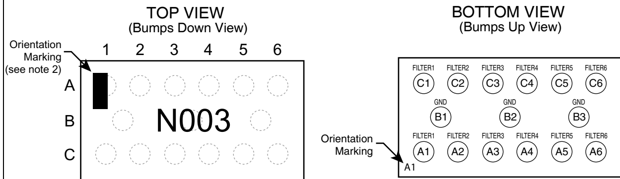
CM1400-03CS/CP CSP Package
