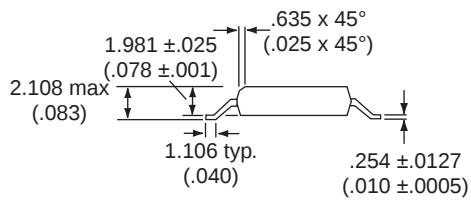
Figure 3. CPC5601 Mechanical Specifications
