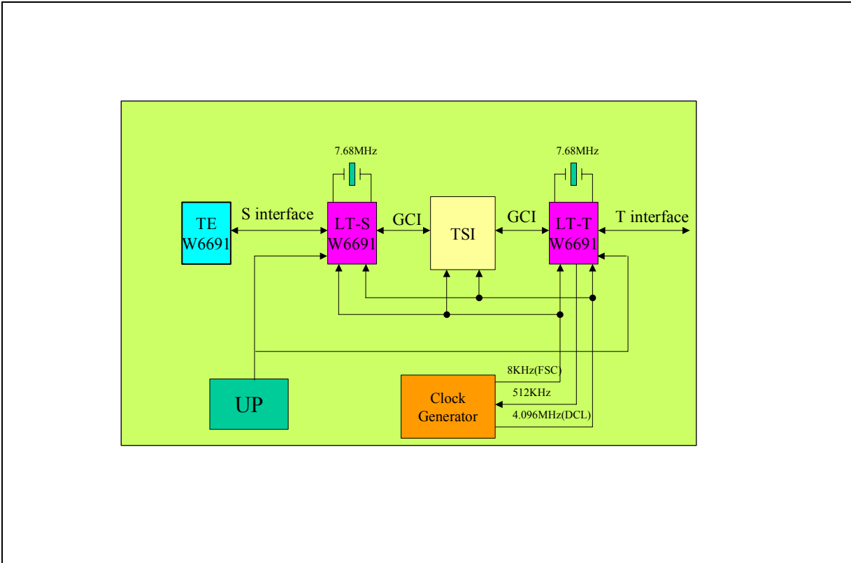
Fig.5.2 ISDN PAXB Application
