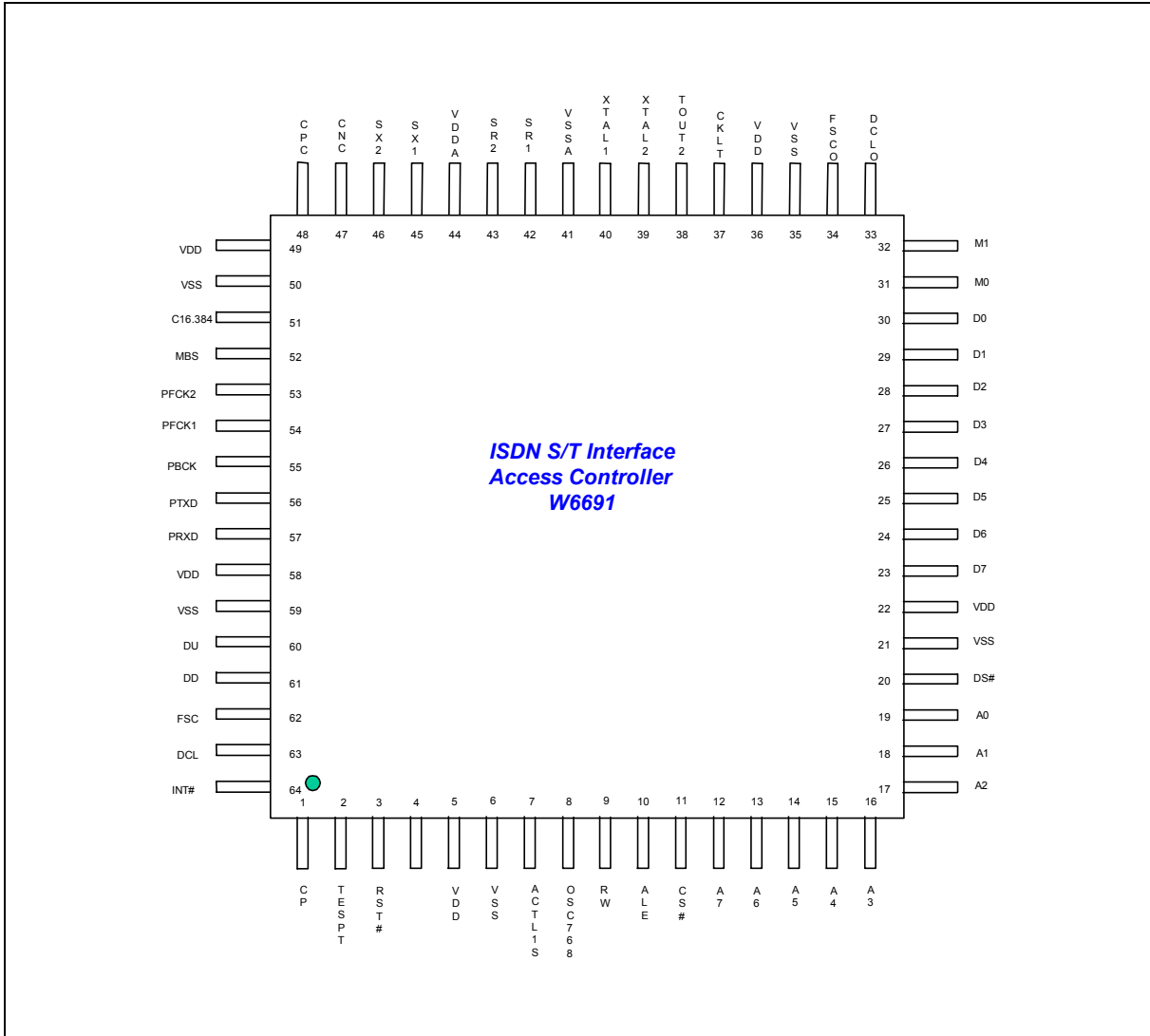
Fig.3.2 W6691 Pin Configuration – Motorola Bus Mode
