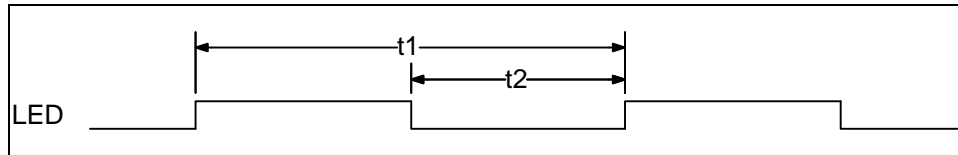
FIGURE 40 – LED OUTPUT TIMING
