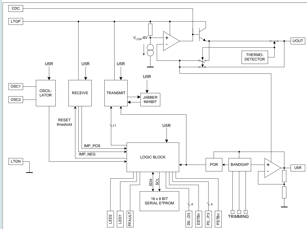
Figure 1 Block diagram
