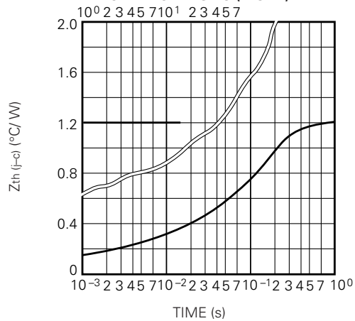
TRANSIENT THERMAL IMPEDANCE CHARACTERISTIC (DIODE)
