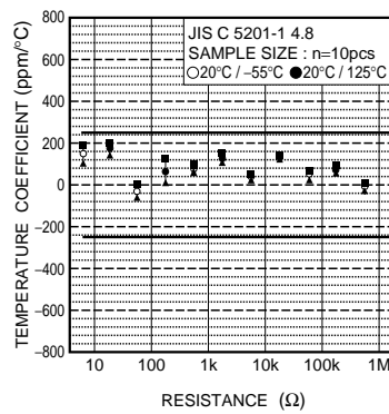
Fig.6 Variation of resistance with temperature
