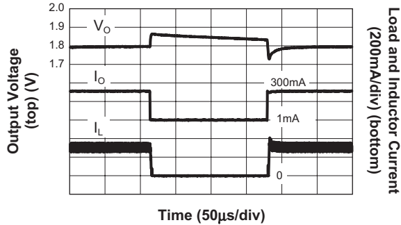
Load Transient Response (1mA to 300mA; V_{IN} = 3.6V ; V_{OUT} = 1.8V ; C_1 = 10\mu F ; C_{FF} = 100pF )
