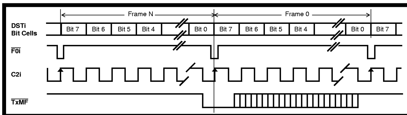
Figure 20 - Functional Timing for Transmit Multiframe Clock
