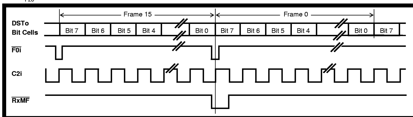
Figure 19 - Functional Timing for Receive Multiframe Clocks
