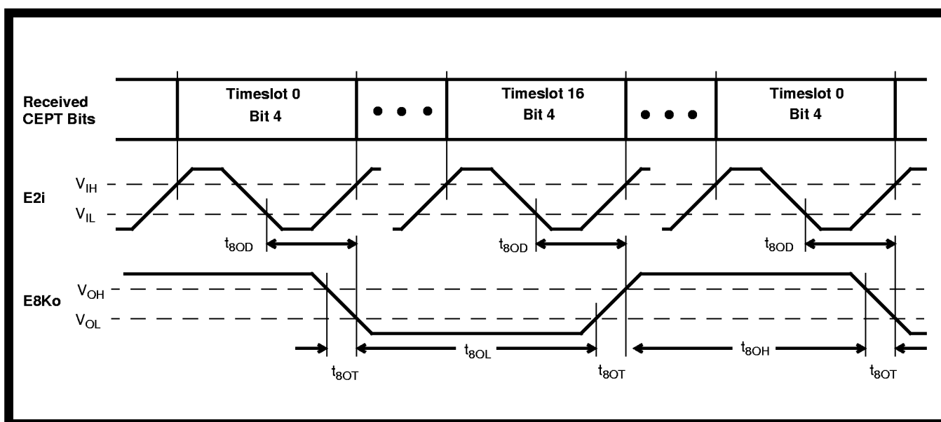
Figure 24 - E8Ko Timing
