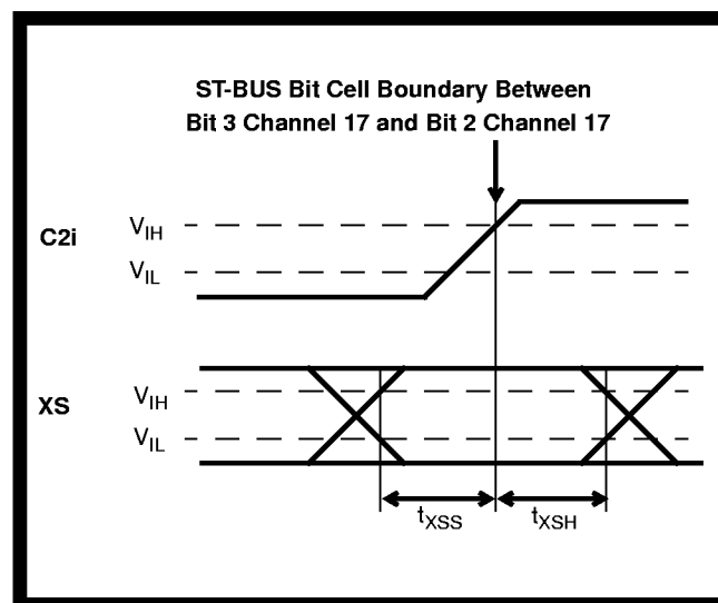
Figure 23 - XS Timing
