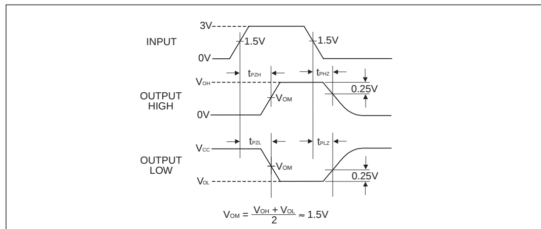
Figure 6. Driver Enable and Disable Timing Waveforms
