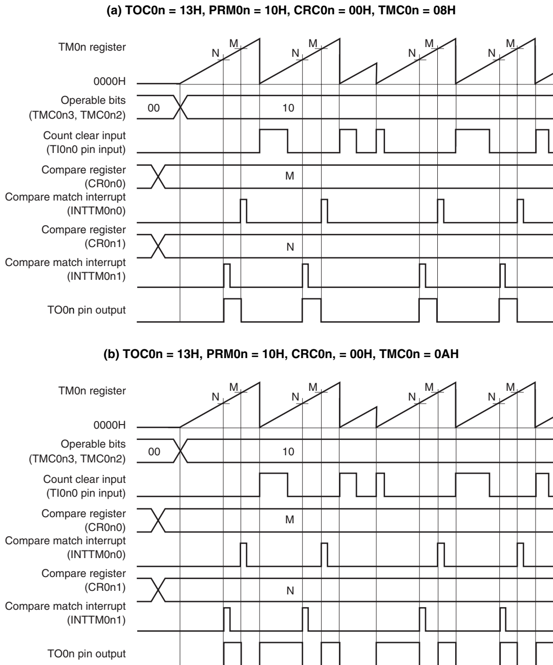
Figure 8-14. Timing Example of Clear & Start Mode Entered by TIO n 0 Pin Valid Edge Input (CR0 n 0 Register: Compare Register, CR0 n 1 Register: Compare Register)
