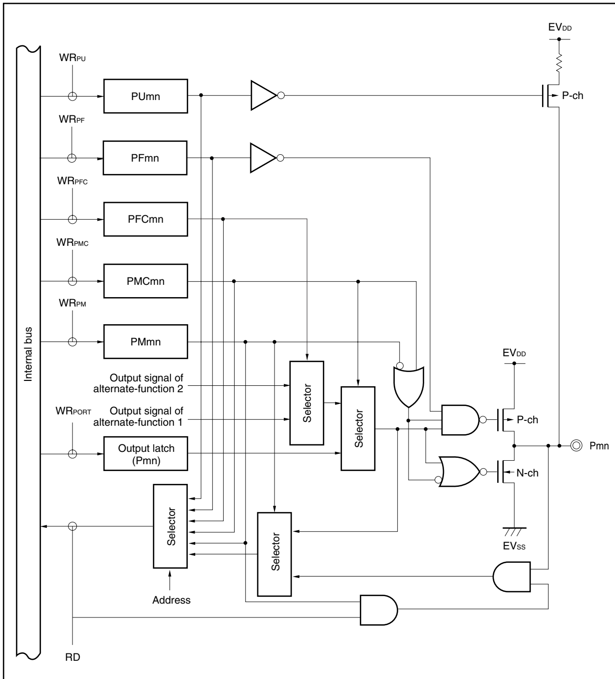
Figure 4-19. Block Diagram of Type E00-UF
