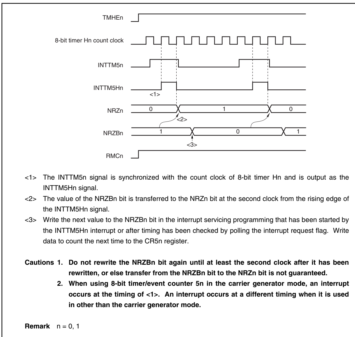
Figure 10-6. Transfer Timing
