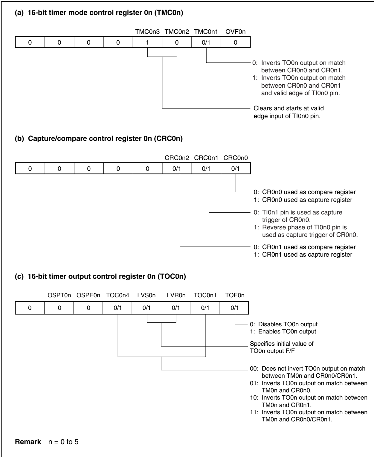
Figure 8-21. Example of Register Settings in Clear &amp; Start Mode Entered by TI0n0 Pin Valid Edge Input (1/2)
