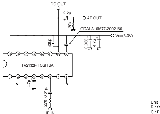
Test Circuit
