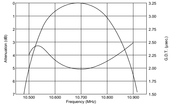
SFELA10M7FALL-B0
