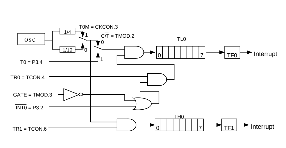
Figure 13. Timer/Counter 0 Mode 3
