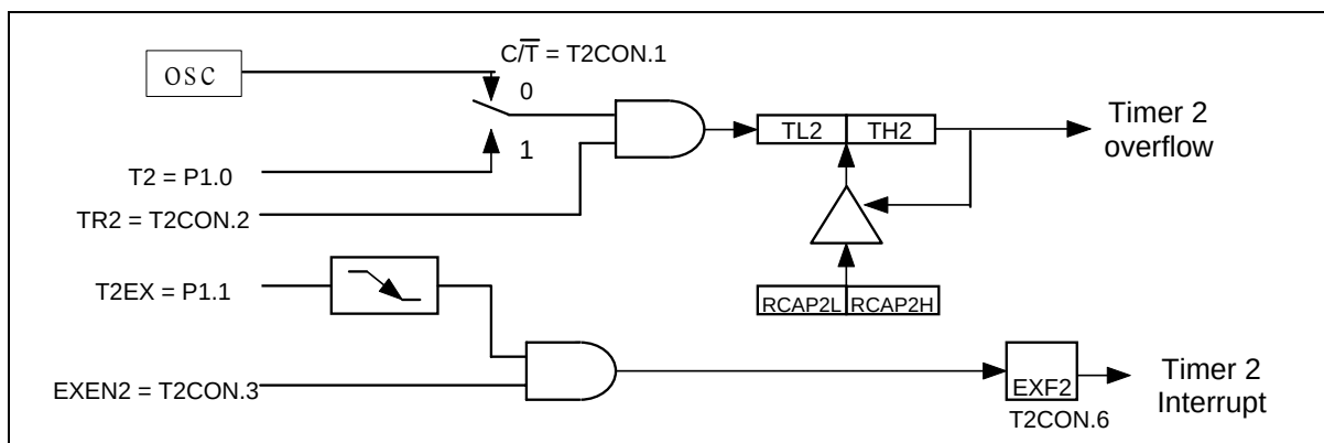
Figure 17. Baud Rate Generator Mode
