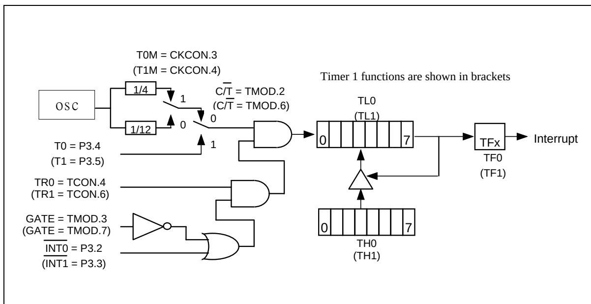
Figure 12. Timer/Counter Mode 2.
