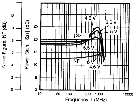
NOISE FIGURE AND POWER GAIN vs. FREQUENCY
