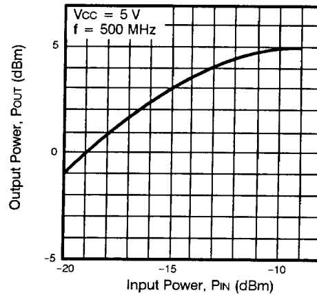
INPUT POWER vs. OUTPUT POWER
