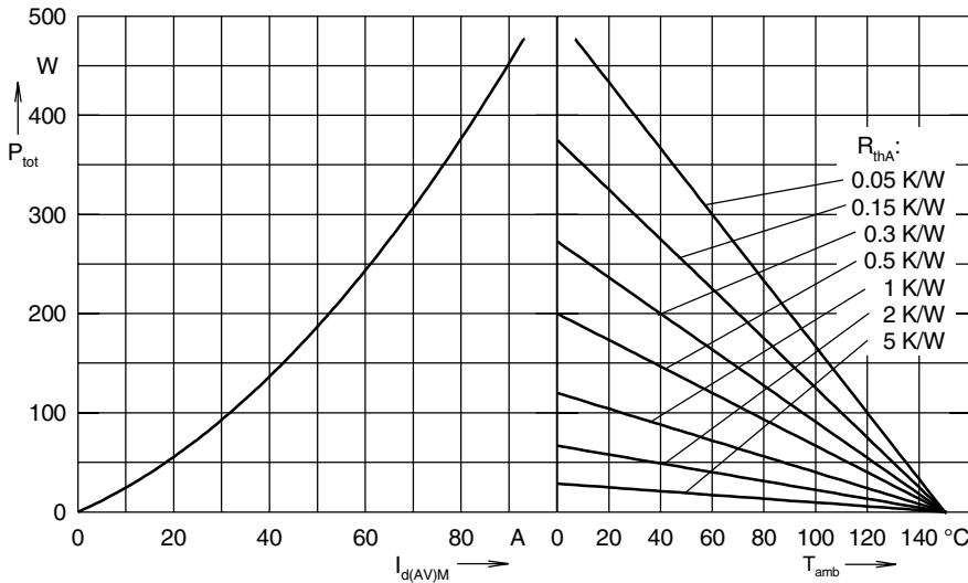
Fig. 4 Power dissipation versus direct output current and ambient temperature, sin 80°
