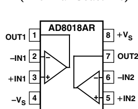
8-Lead SOIC (Thermal Coastline)
