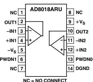
14-Lead TSSOP
