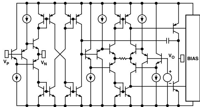
Figure 4. Simplified Schematic
