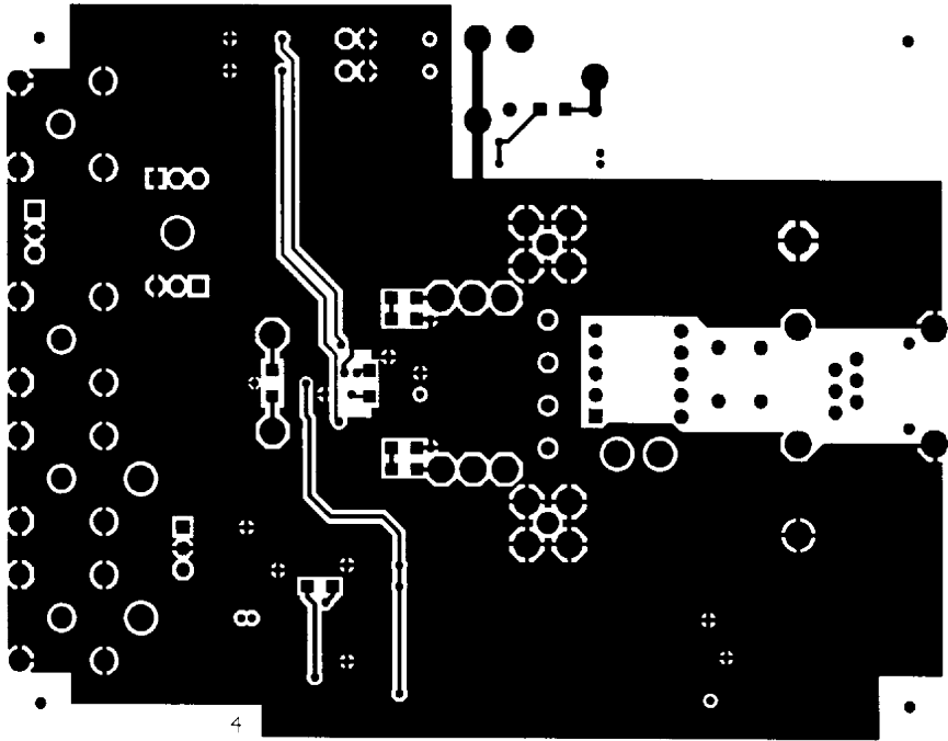
Figure 18. Layer 4—Secondary Side
