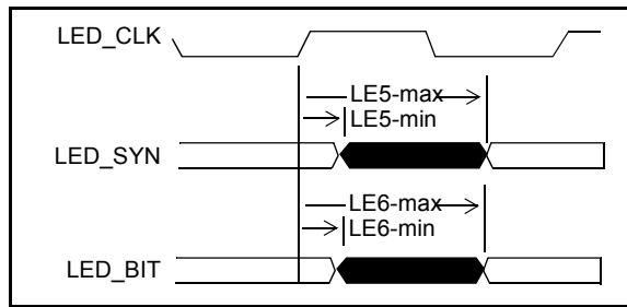
Figure 22 - AC Characteristics – LED Interface
