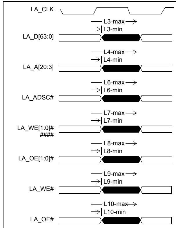
Figure 19 - Local Memory Interface – Output valid delay timing
