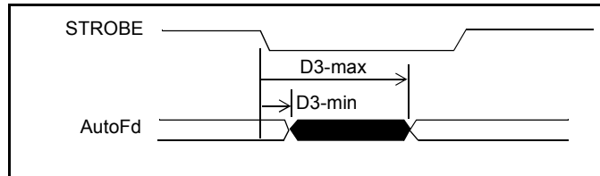
Figure 30 - Serial Interface Output Delay Timing
