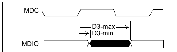
Figure 26 - MDIO Output Delay Timing
