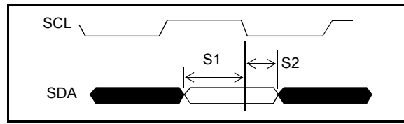
Figure 27 - I 2 C Input Setup Timing
