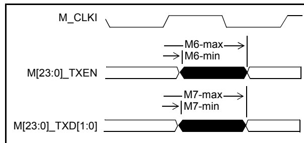
Figure 20 - AC Characteristics - Reduce Media Independent Interface
