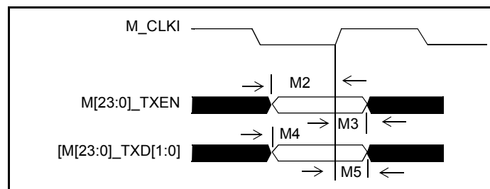
Figure 21 - AC Characteristics – Reduced media independent Interface
