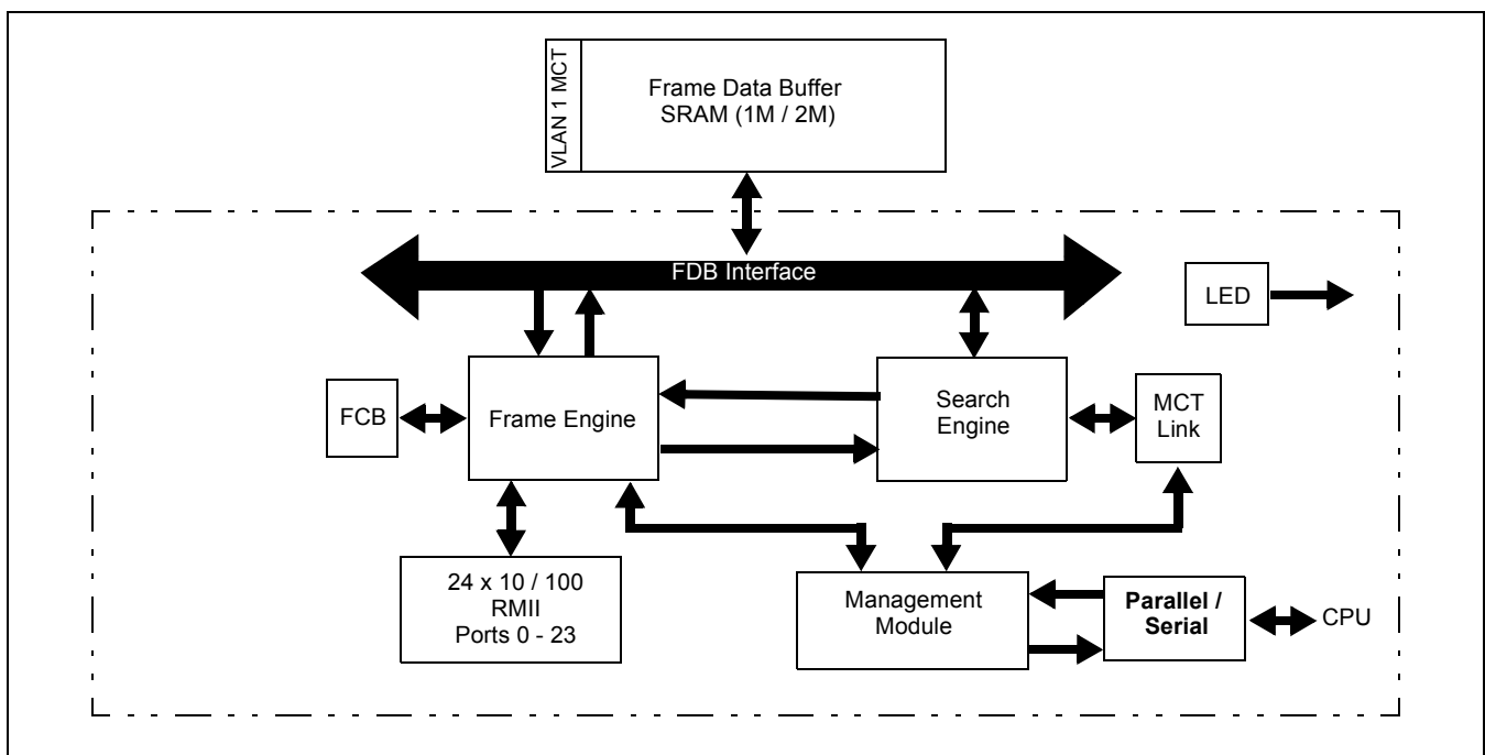
Figure 1 - MVTX2602 System Block Diagram
