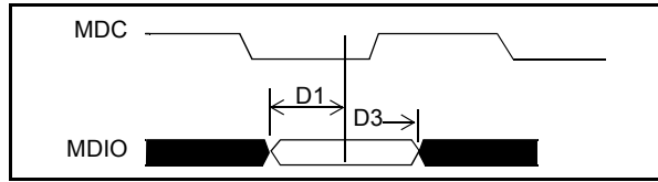
Figure 25 - MDIO Input Setup and Hold Timing
