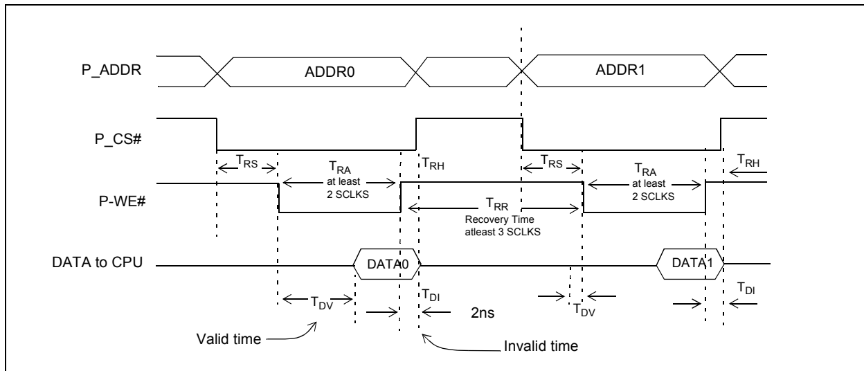
Figure 17 - Typical CPU Timing Diagram for a CPU Read Cycle
