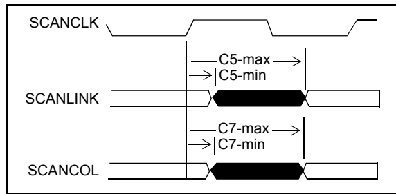
Figure 23 - SCANLINK SCANCOL Output Delay Timing
