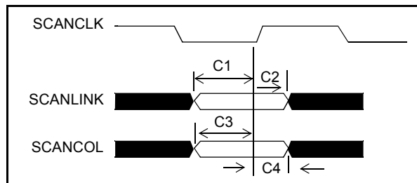
Figure 24 - SCANLINK, SCANCOL Setup Timing
