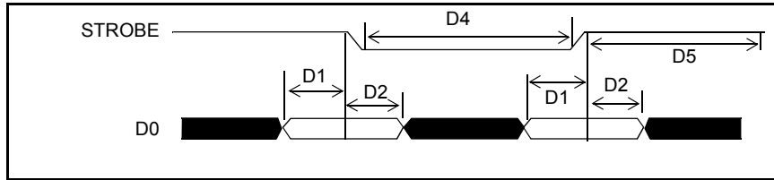
Figure 29 - Serial Interface Setup Timing
