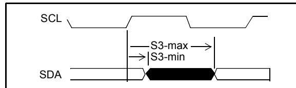
Figure 28 - I 2 C Output Delay Timing
