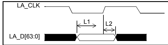
Figure 18 - Local Memory Interface – Input setup and hold timing
