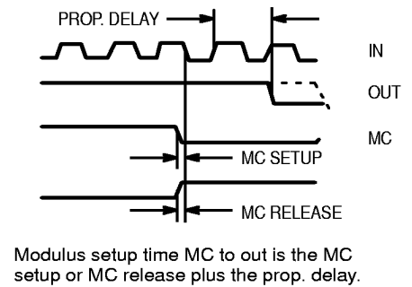
Figure 2. Modulus Setup Time
