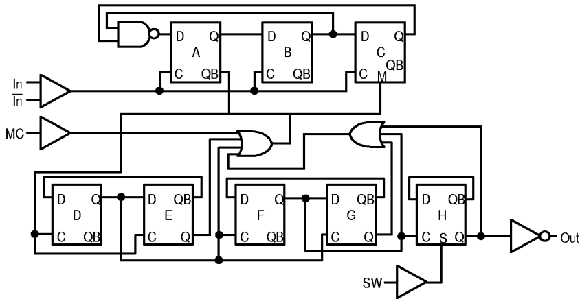
Figure 1. Logic Diagram (MC12034A)
