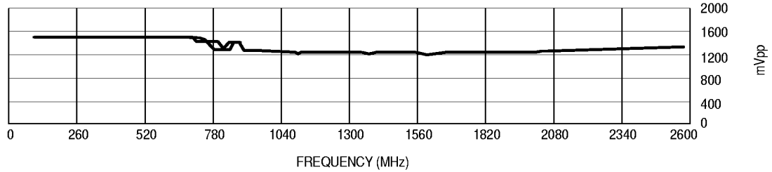
Figure 6. Output Amplitude versus Input Frequency
