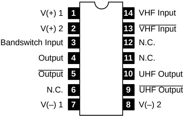
Pin Connection Diagram
