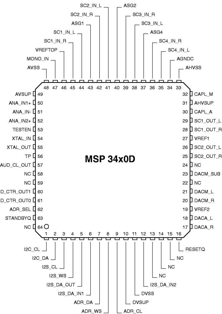
Fig. 9–10: 64-pin PLQFP package
