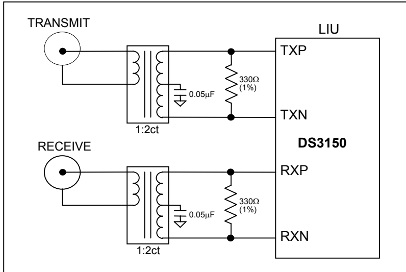
Figure 1. Line-Side Circuitry
