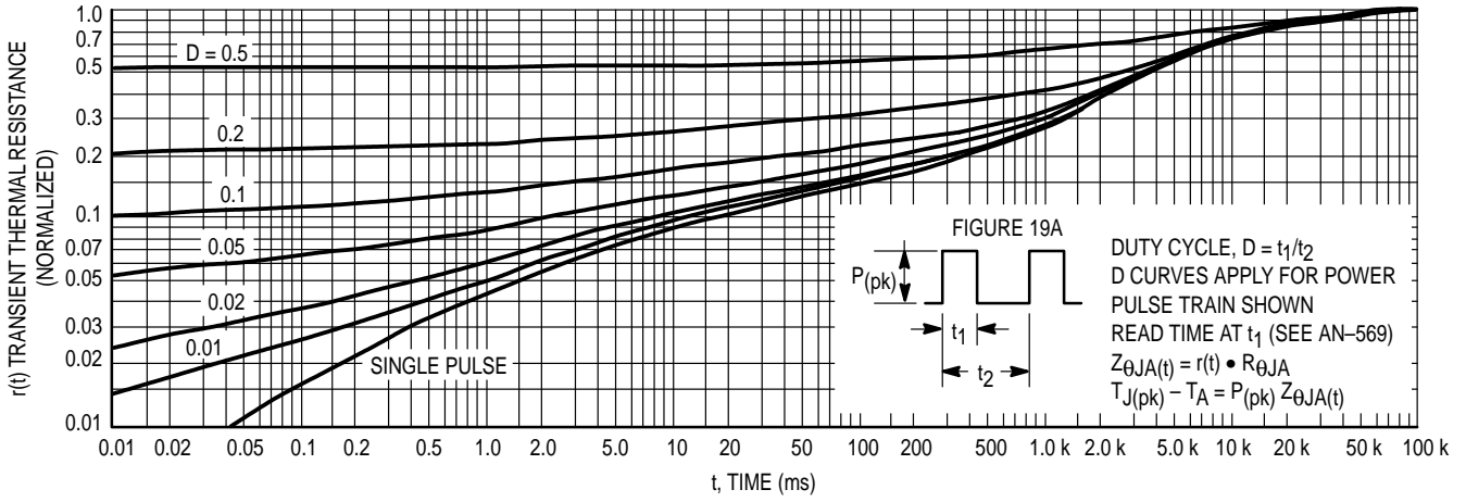
Figure 19. Thermal Response
