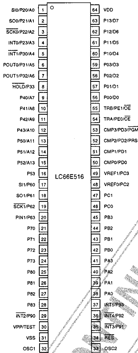
Figure 11. LC66E516 pinout
