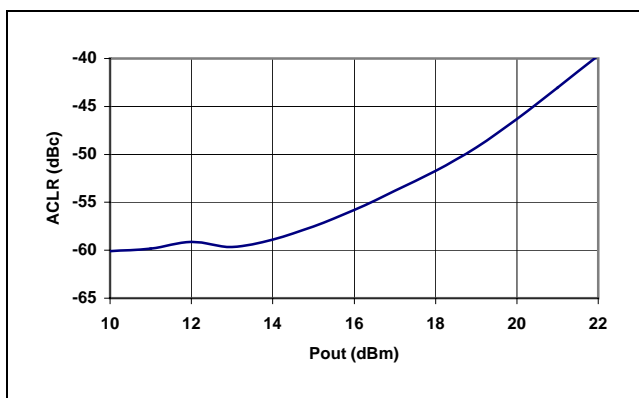
Figure 17. Typical ACLR vs P OUT @ 2.14 GHz, 5 MHz Offset, 25 °C (Circuit Match for Optimum ACPR)
