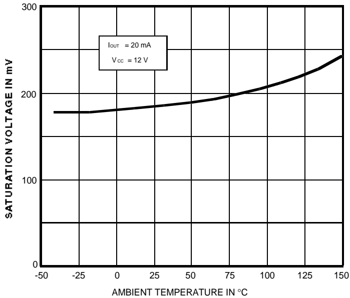
OUTPUT SATURATION VOLTAGE
