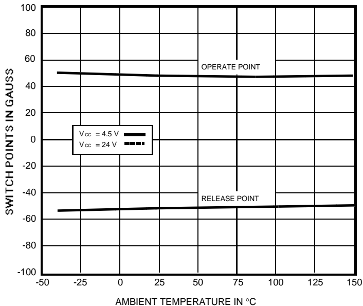
A3281* SWITCH POINTS
