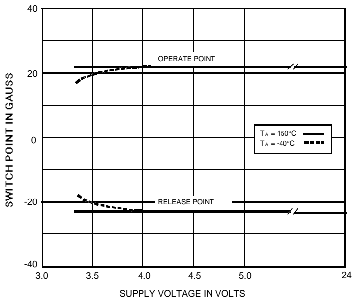
A3280* SWITCH POINTS
