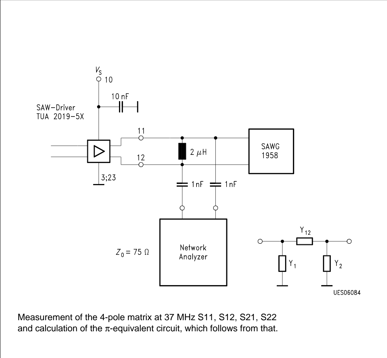
Test Circuit 4
