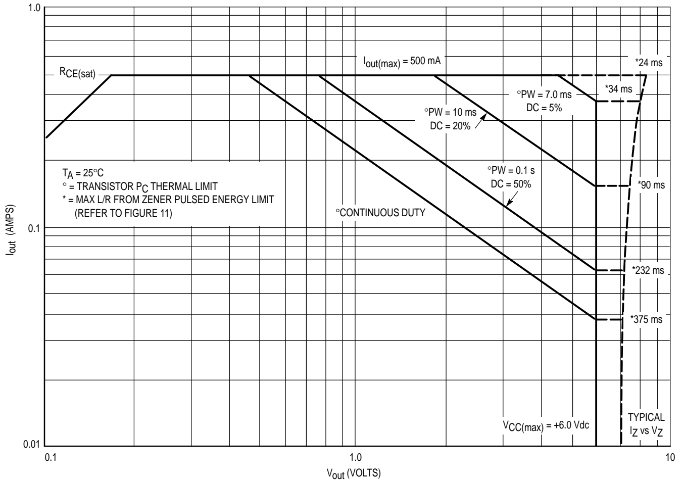
Figure 10. Safe Operating Area
