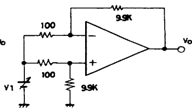
(3) CMRR, V_{ICM}
